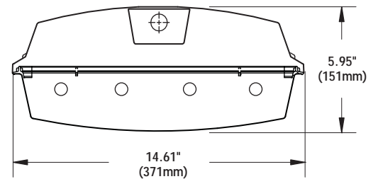
4 Lamp T5
